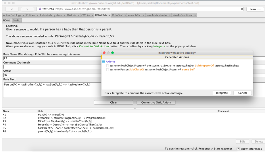
Fig. 1. The ROWLTab interface with generated axioms.
